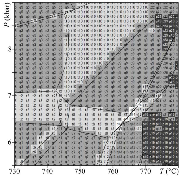
Appendix 8. P - T pseudosections calculated with the barycentric coordinate system compositional space (based on Eq. 9.1) in the system NCKFMASH using the Cartesian formula (cation) and the TC book for the same bulk composition as shown in Fig. 9a (Table 4g). The P - T pseudosection from Fig. 9b is superimposed onto the diagram (thin lines).
