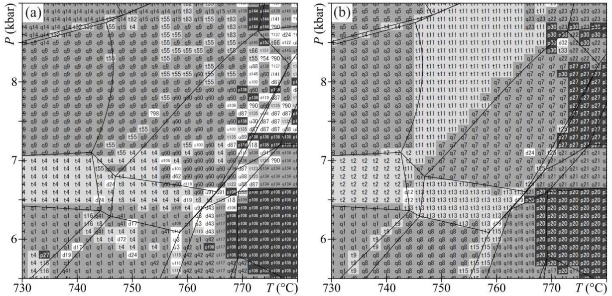
Appendix 7. P - T pseudosections calculated in the system NCKFMASH using the Cartesian formula (cation) and the TC book for (a) the same bulk composition as shown in Fig. 9a (Table 4g) and (b) the bulk composition provided in (a) multiplied by 10 (Table 4h). The P - T pseudosection from Fig. 9b is superimposed onto the diagrams (thin lines).
